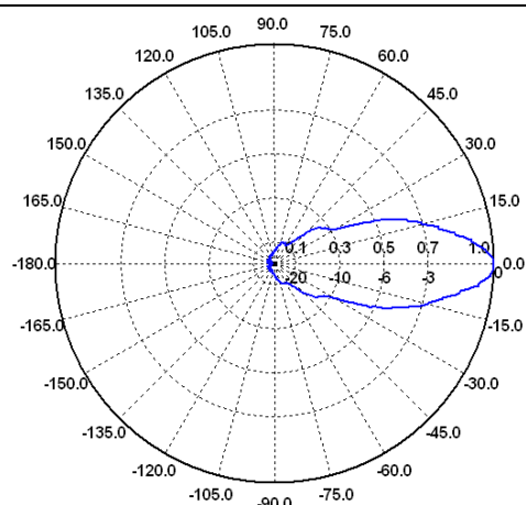
E-Ebene / E-Plane 16 GHz
