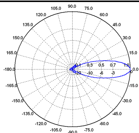
H-Ebene / H-Plane 14 GHz
