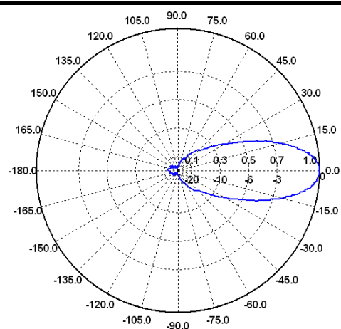
H-Ebene / H-Plane 8 GHz
