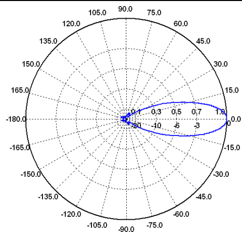
H-Ebene / H-Plane 12 GHz
