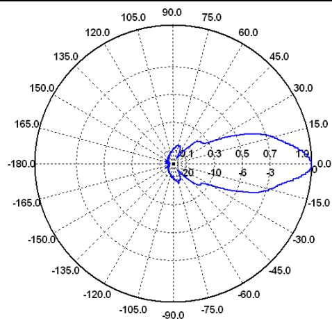
E-Ebene / E-Plane 15 GHz
