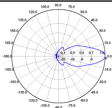
E-Ebene / E-Plane 11 GHz
