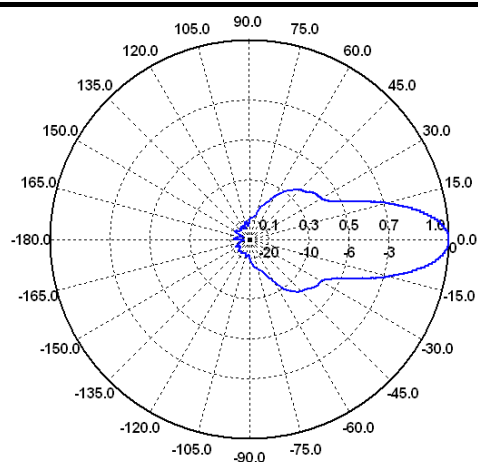
E-Ebene / E-Plane 8 GHz
