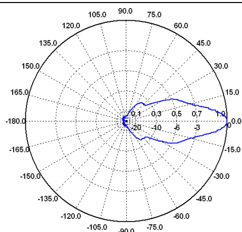
E-Ebene / E-Plane 13 GHz
