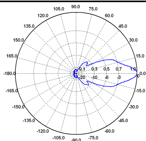
E-Ebene / E-Plane 14 GHz
