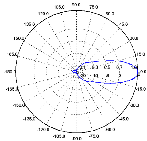
H-Ebene / H-Plane 9 GHz
