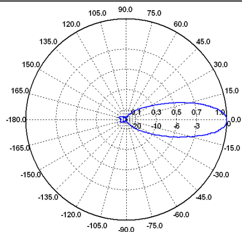
H-Ebene / H-Plane 10 GHz
