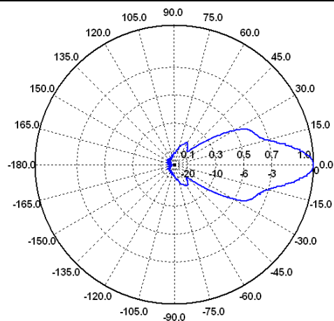
E-Ebene / E-Plane 12 GHz
