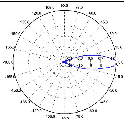
H-Ebene / H-Plane 16 GHz
