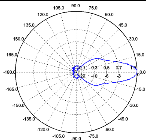
E-Ebene / E-Plane 10 GHz
