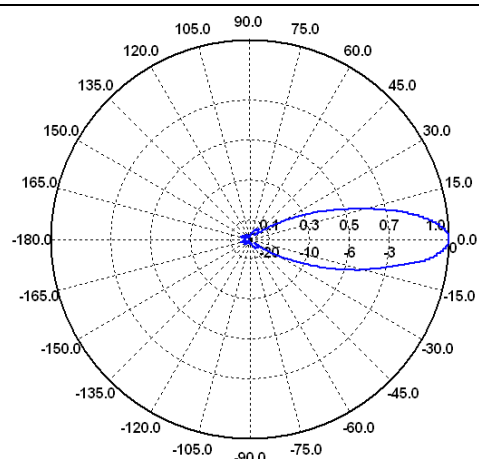
H-Ebene / H-Plane 13 GHz
