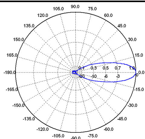
H-Ebene / H-Plane 11 GHz
