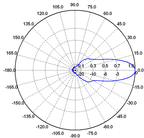
E-Ebene / E-Plane 9 GHz
